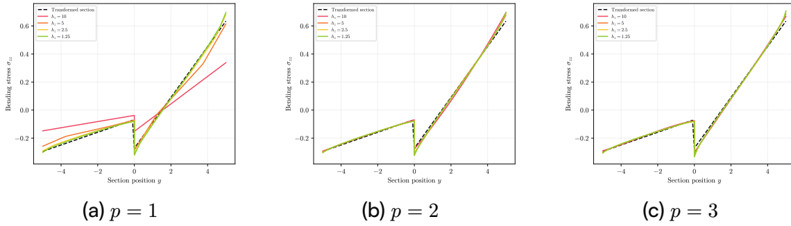
Figure 16: Body force: bending stress through the clamped section, where the moment (and the interface jump) is largest.
