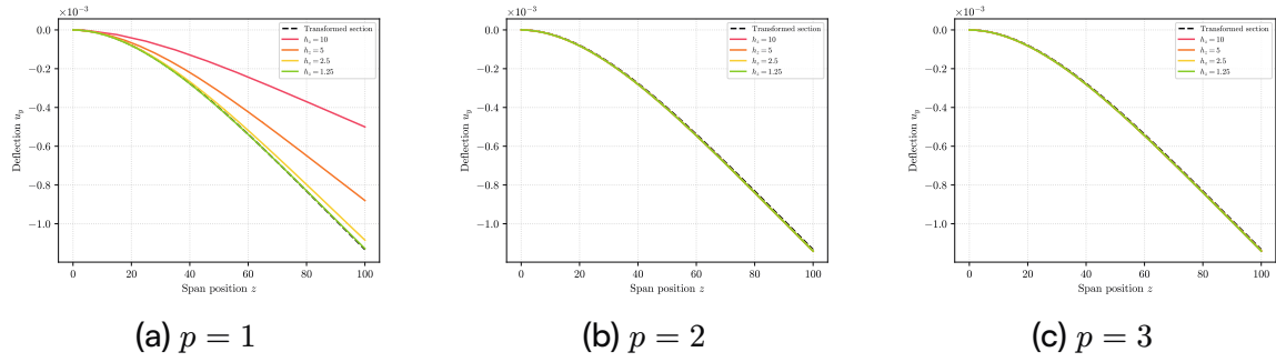
Figure 8: Gravity: deflection along the interface line — coarse→fine sweep per degree vs the transformed section.
