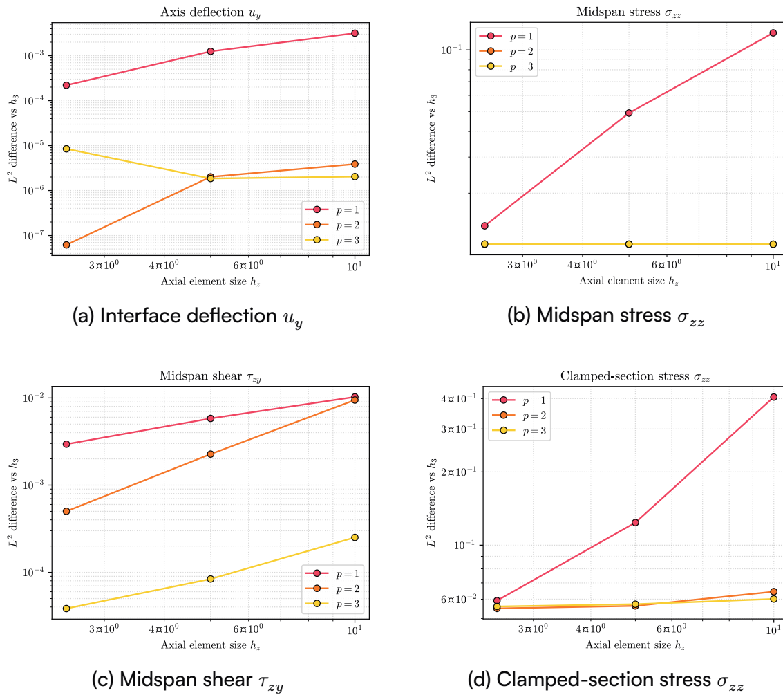
Figure 12: Gravity: full-span line-probe absolute L2 self-convergence. Each degree is compared against its own h_3 profile; the h_3 point is omitted because its self-error is zero.
