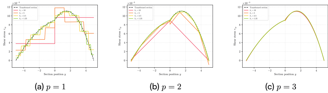
Figure 15: Body force: shear stress through the midspan section — continuous across the interface, with its maximum at the neutral axis.
