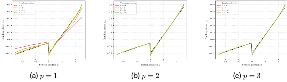
Figure 21: Pressure: bending stress through the clamped section, where the moment (and the interface jump) is largest.
