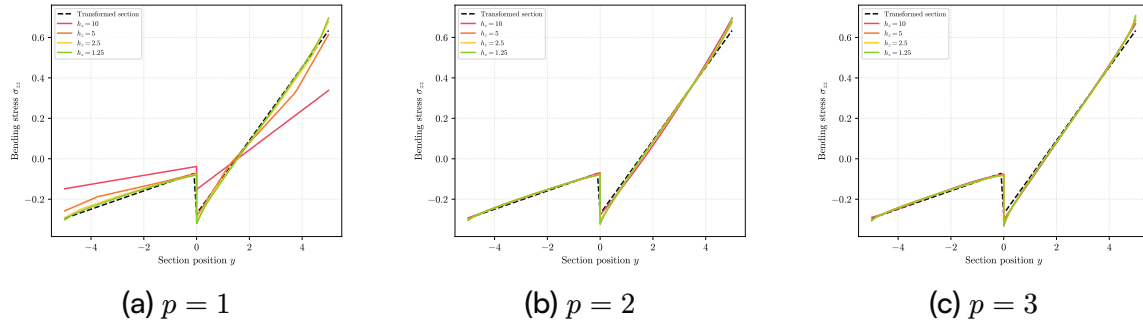
Figure 11: Gravity: bending stress through the clamped section, where the moment (and the interface jump) is largest.
