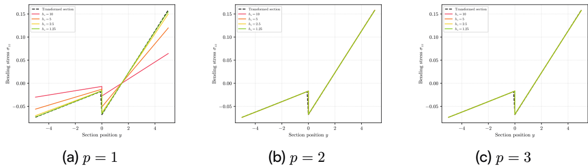
Figure 14: Body force: bending stress through the midspan section — the closed form jumps by the modular ratio at the material interface ( y = 0 ).
