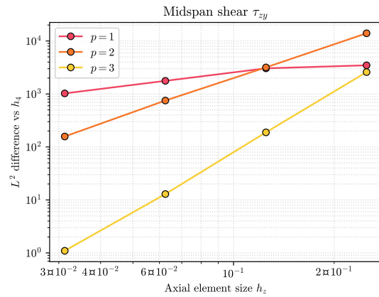
a(d) Midspan shear \tau_{zy}
