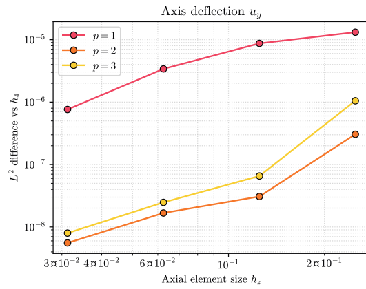
a(a) Axis deflection u_y
