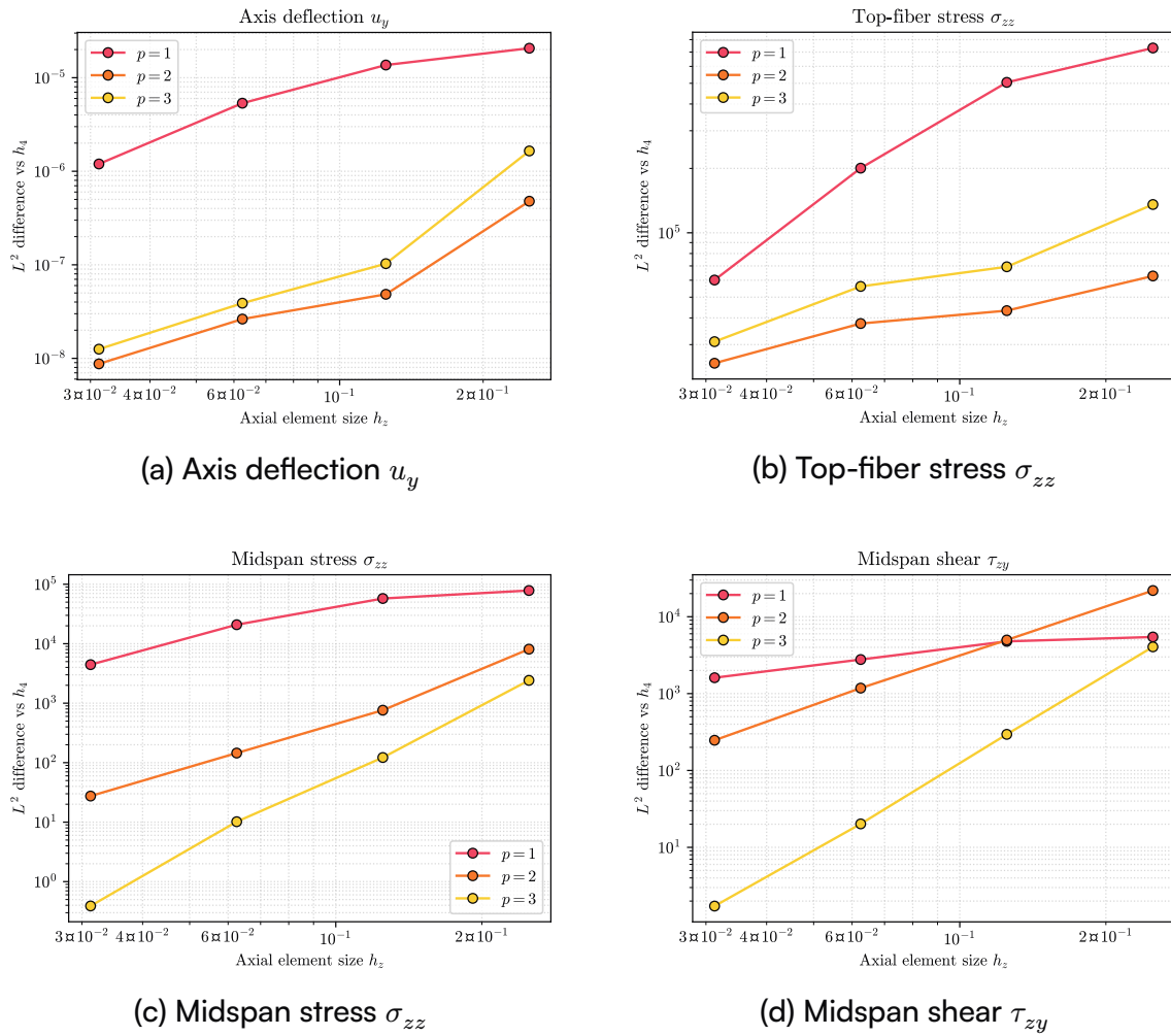
Figure 17: Body force: full-span line-probe absolute L2 self-convergence. Each degree is compared against its own h_4 profile; the h_4 point is omitted because its self-error is zero.
